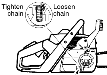
Adjusting Wheel
